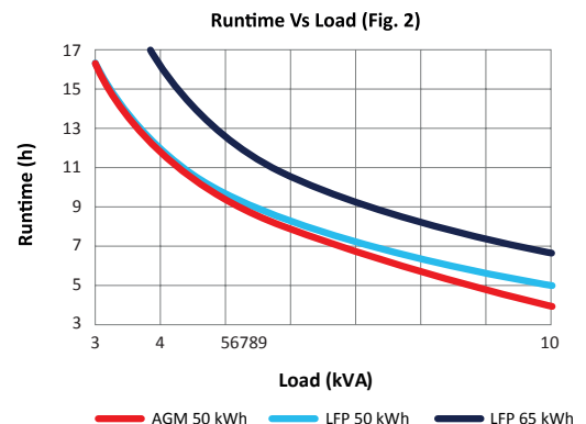
FIREFLY CYGNUS 3 <100kVA
